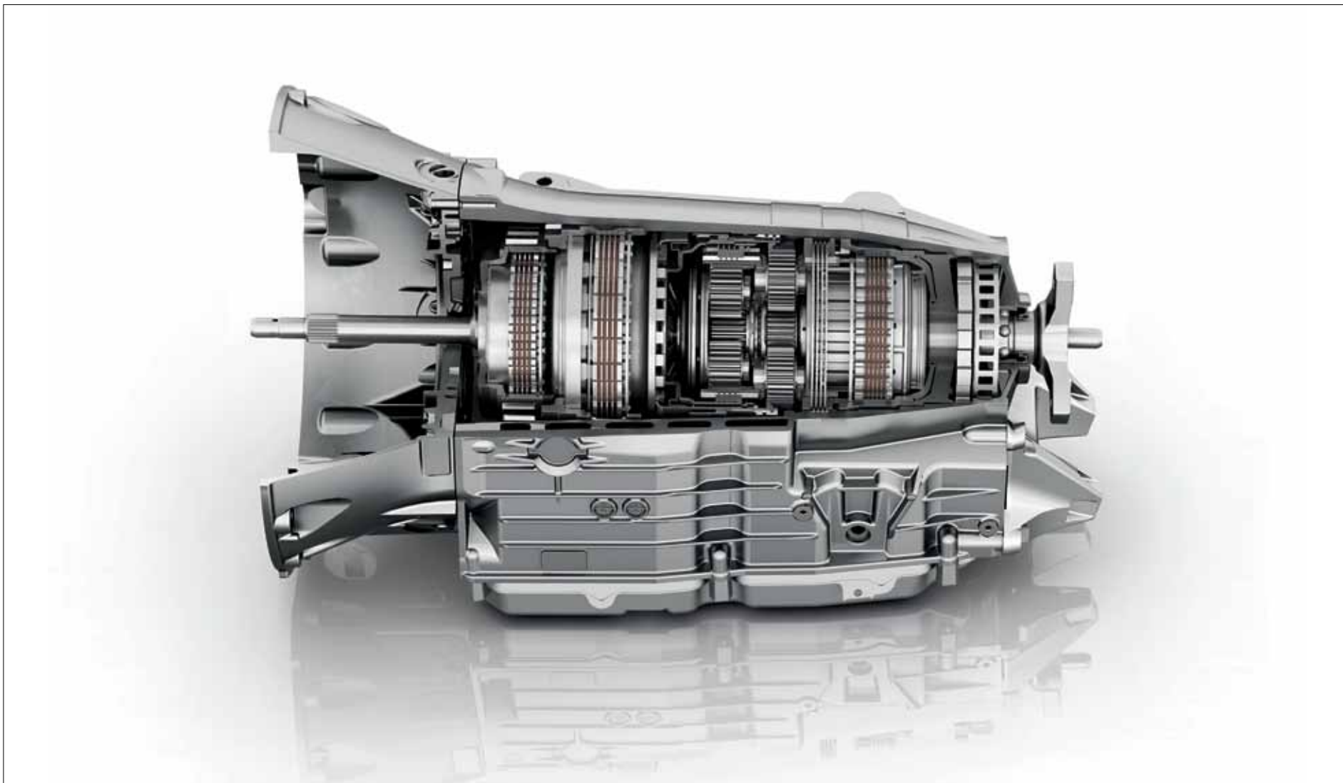
The 7G-TRONIC PLUS automatic transmission; one of over 18 million automatic transmissions produced in a period spanning more than 50 years.
