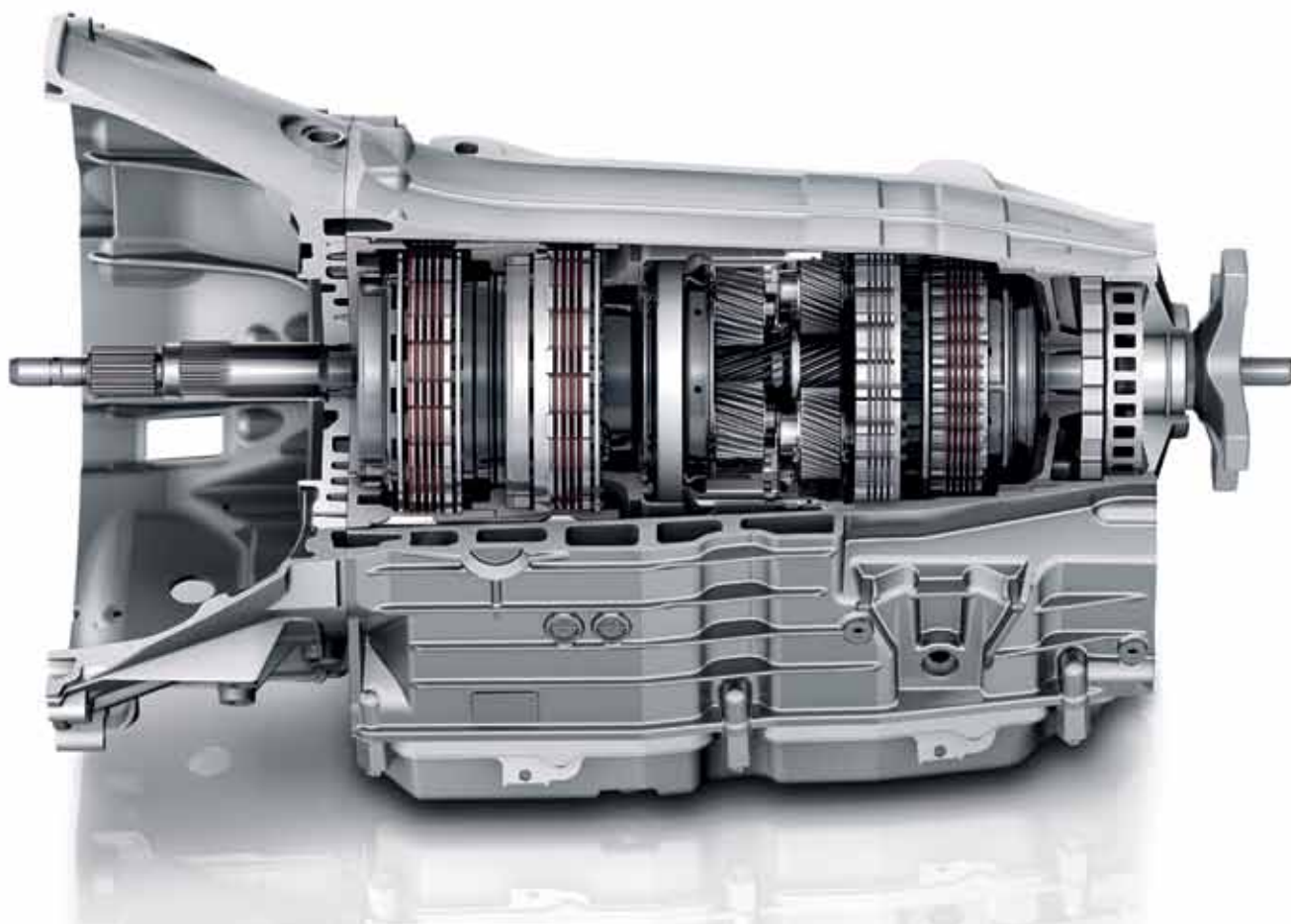
The 7G-TRONIC PLUS: one of over 18 million automatic transmissions produced in a period spanning more than 50 years.
